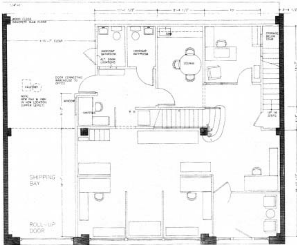
REVISED LOWER FLOOR PLAN
