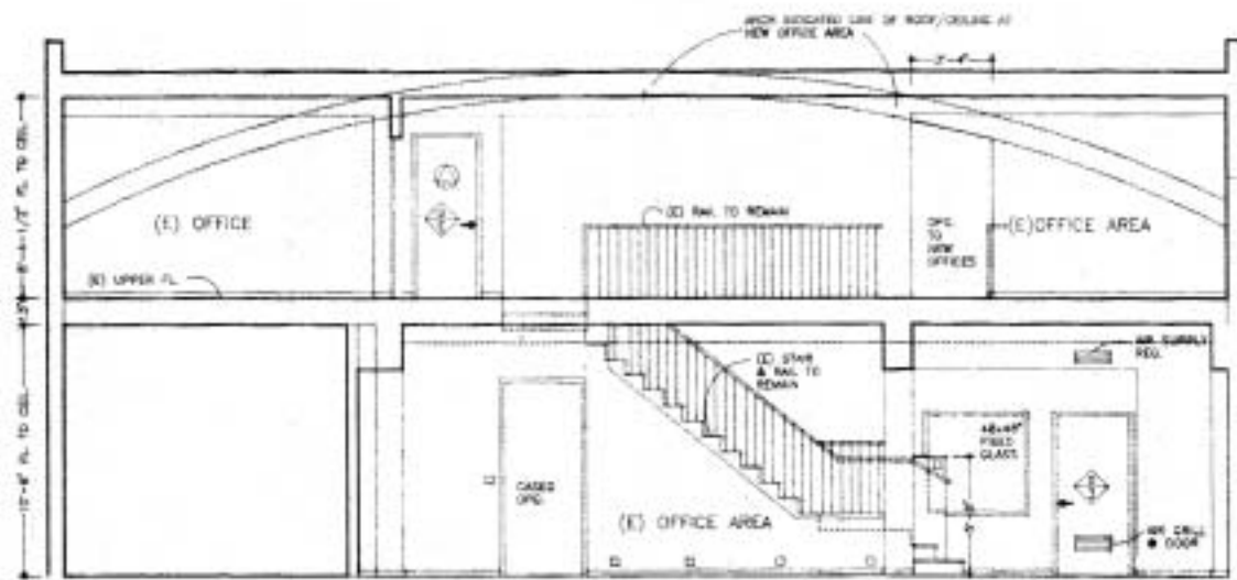
SECTION THRU EXISTING OFFICE SPACE
