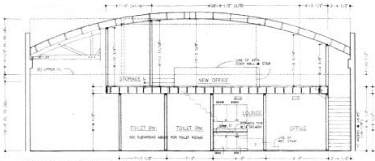
SECTION THRU NEW OFFICE SPACE
